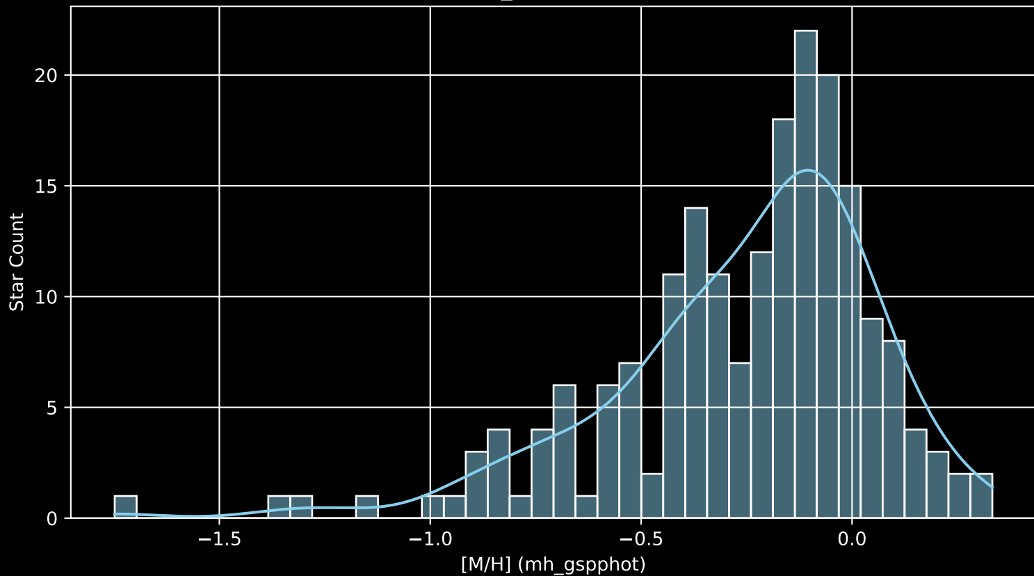
APOGEE DR17 Field: [064-46_MGA [M/H] (mh_gspphot) (n= 198)
