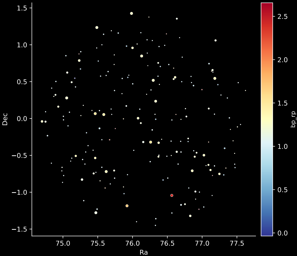
APOGEE DR17 Field: [064-46_MGA] Stars: 202
