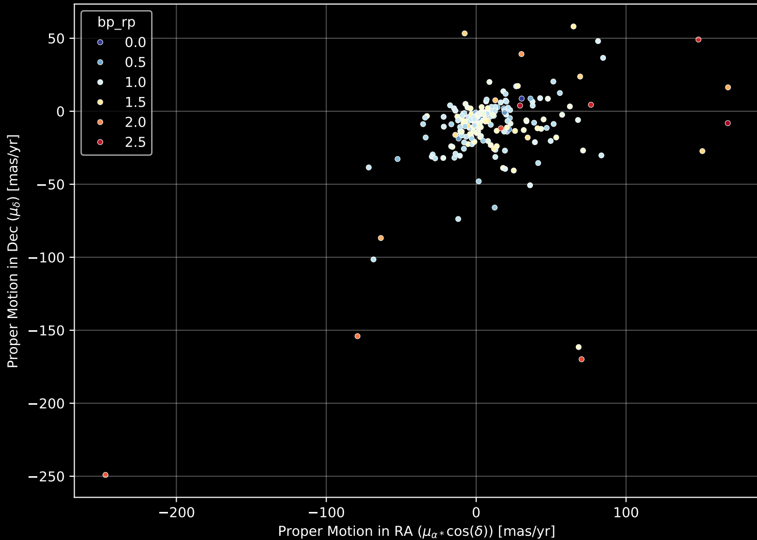
APOGEE DR17 Field: [064-46_MGA] Proper Motion Diagram (n= 202)
