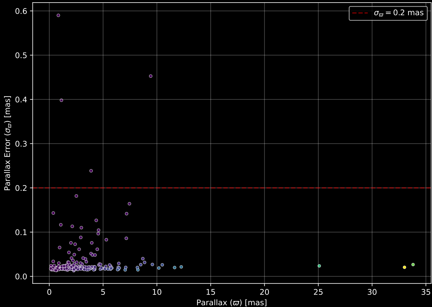
APOGEE DR17 Field: [064-46_MGA] Parallax Quality (n= 202)
