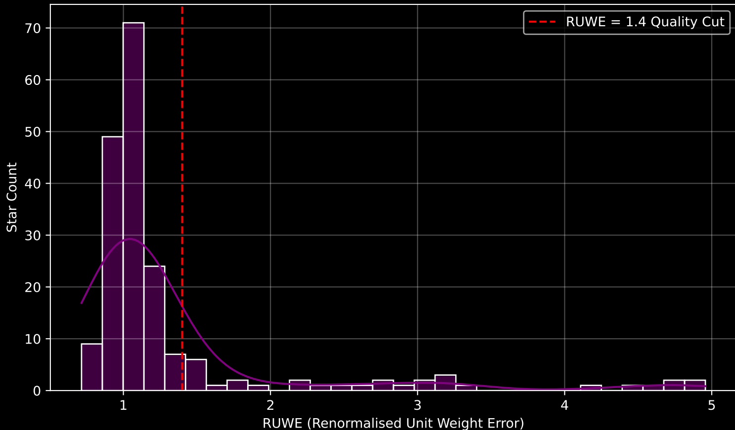
GAPOGEE DR17 Field [064-46_MGA] RUWE Distribution (n= 191)
