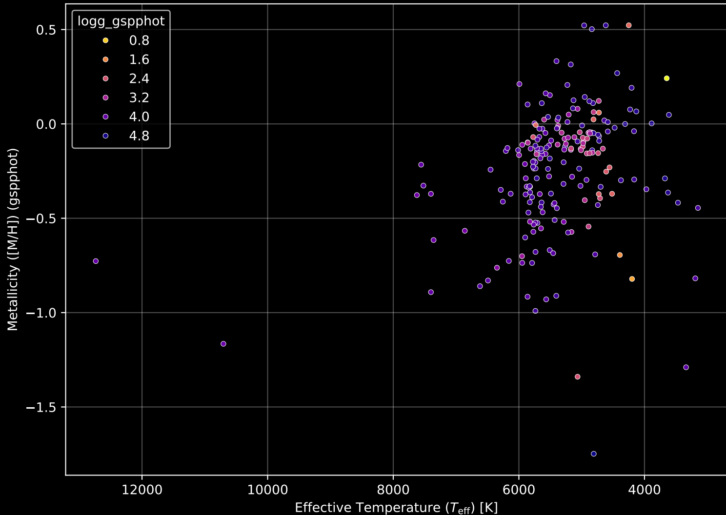
APOGEE DR17 Field: [064-46_MGA] Stellar Population Parameters (n= 202)
